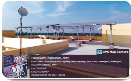
20 kWp Grid Connected SPV Power Plant at Govt. College, Walgarh Jhunjhunu)
